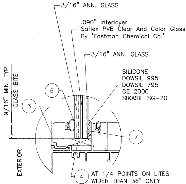
GLASS TYPE 'A' 7/16" OVERALL LAM. GLASS
